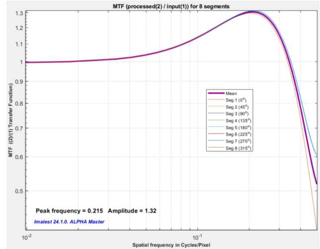
Figure 30. Filter transfer function for \sigma = 0.7 , Radius = 1, Amount = 2; R1A2.
