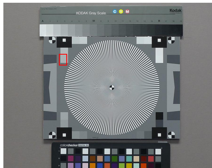
Figure 11. Typical image (cropped) including Siemens star and slanted-edges to the left and right of the star.
