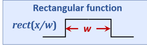
Figure 19. rect function
