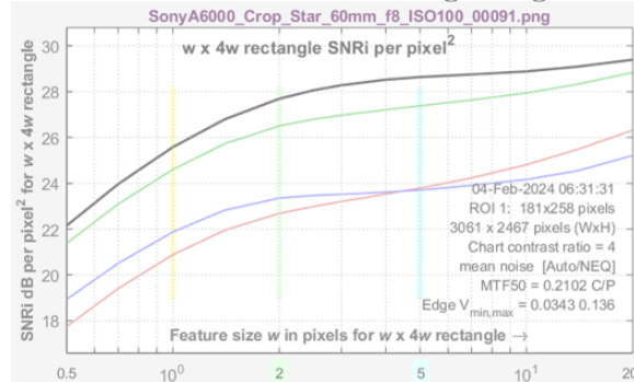
Figure 21a. SNR_i per pixel 2 for a sharp, low-noise (ISO 100) image
