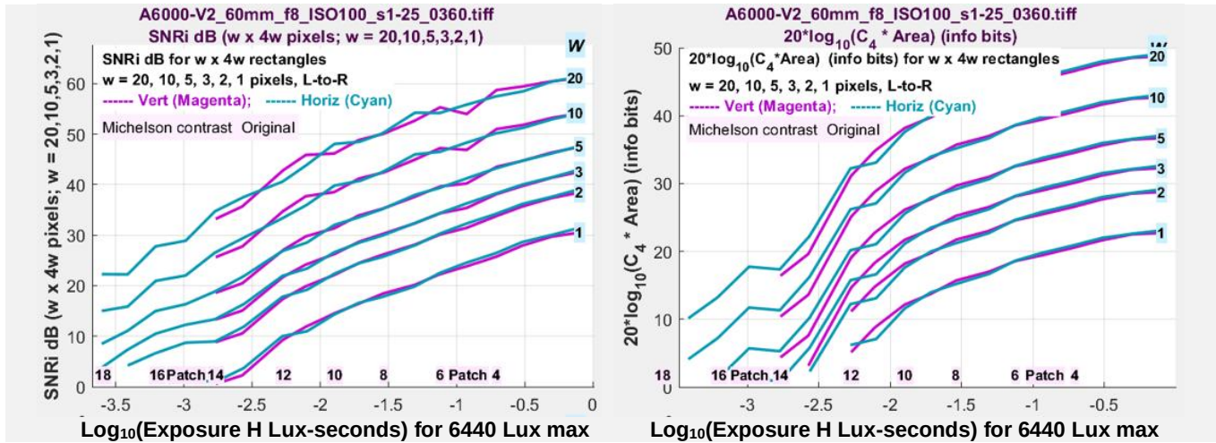
Figure 32. SNR_i dB and 20 \times \log_{10}(C_4 \times \text{Area}) as a function of exposure
