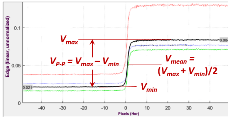
Figure 4. Slanted-edge amplitudes (voltages, V )
