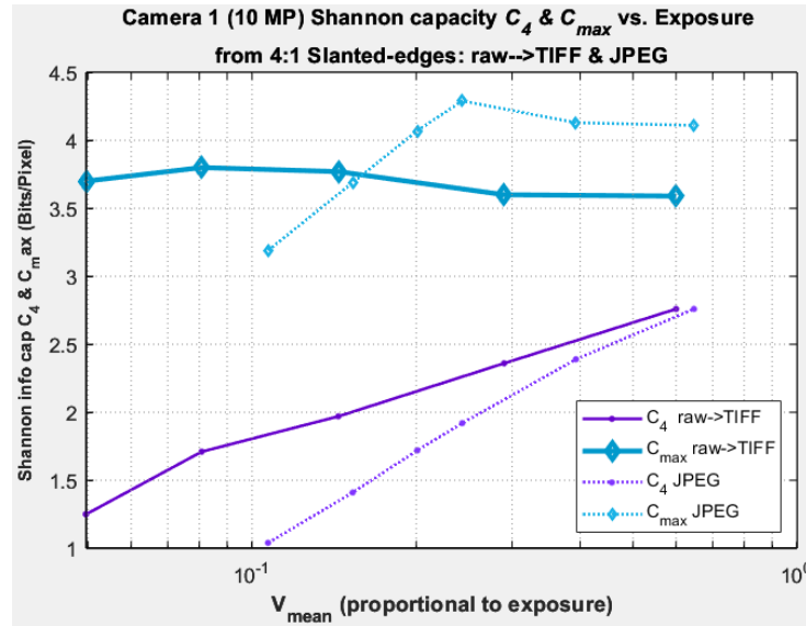
Figure 9. C_4 and C_{max} for minimally processed raw→TIFF and JPEG images for a 10 MP compact camera. C_{max} is consistent for the raw→TIFF image. C_4 is useful for quantifying low light performance.
