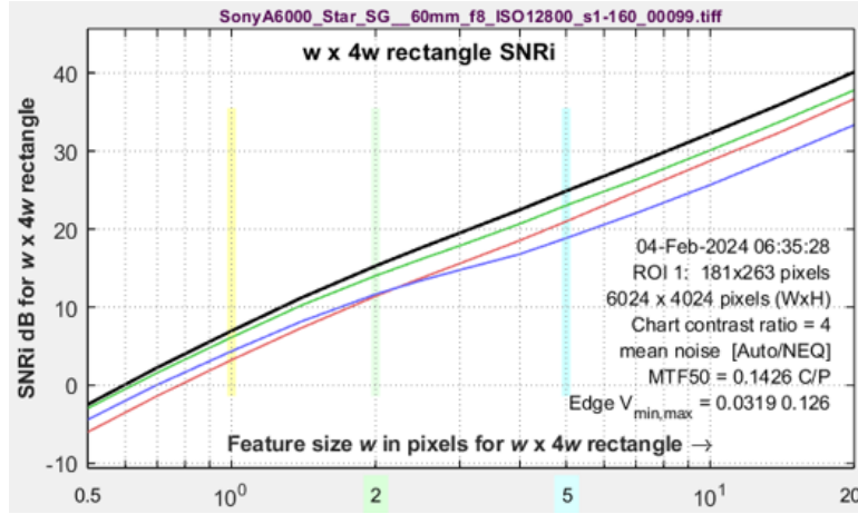
Figure 24. SNR_i for noisy ISO 12800 image (above)
