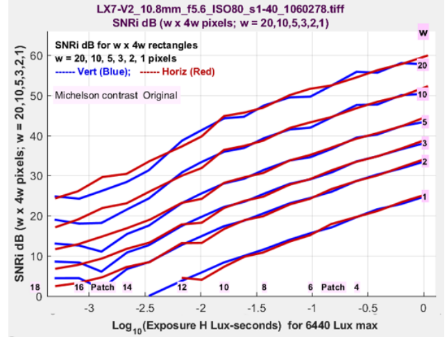
Figure 20a. SNR_i for w \times 4w rectangles with w = 1, 2, 3, 5, 10 & 20 pixels for compact camera.
