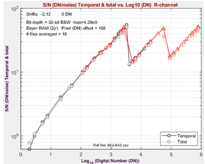
Figure 10. Cyclic response of Signal-to-Noise Ratio for HDR sensor
