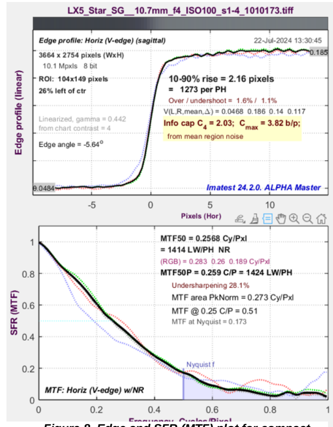
Figure 8. Edge and SFR (MTF) plot for compact digital camera for an unsharpened TIFF from raw. Upper: Mean edge \mu_s(x) ; Lower: SFR(f) .
