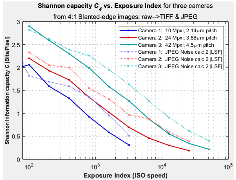
Figure 12. Information capacity, C_4 , from 4:1 slanted-edge images. Solid lines for raw→TIFF images; Dotted lines for JPEGs. Note that increasing the Exposure Index decreases the exposure (total light reaching the image sensor).
