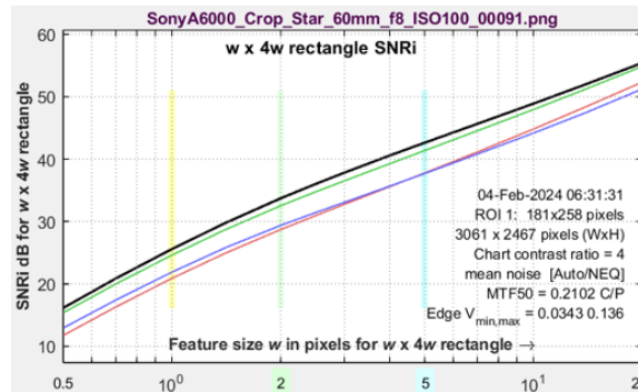
Figure 20. SNRi as a function of feature size w (in w \times 4w rectangles) for a sharp, low-noise (ISO 100) image for R,G,B,Y channels
