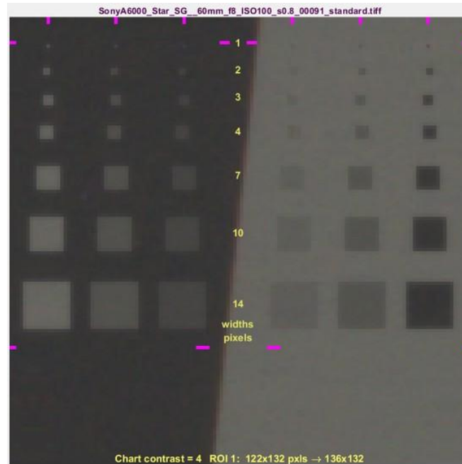
Figure 22. Low noise image, ISO 100.
