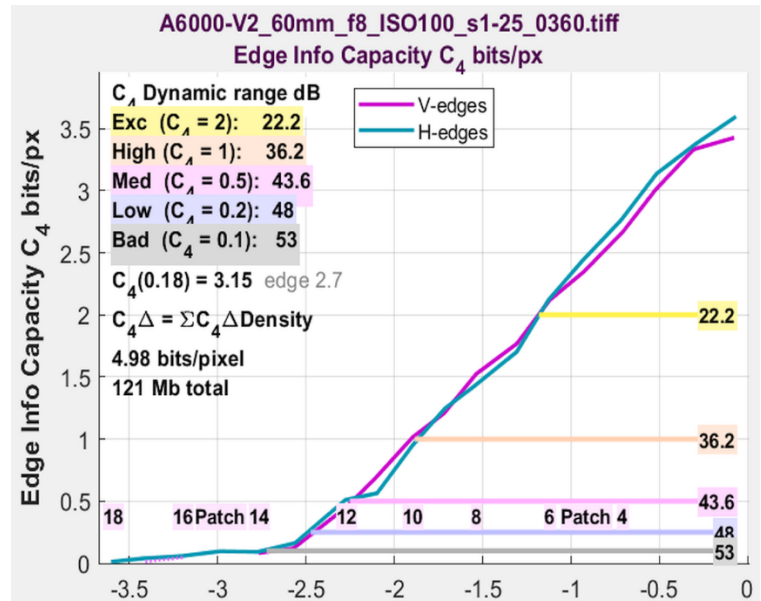
Figure 31. \log_{10}(\text{Exposure } H \text{ Lux-seconds}) for 6440 Lux max from InfoDR chart
