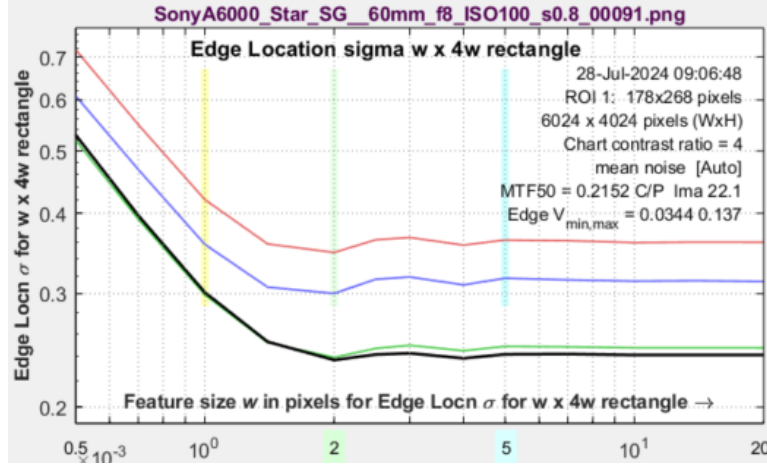
Figure 26. Object location \sigma for a sharp, low-noise (ISO 100) image
