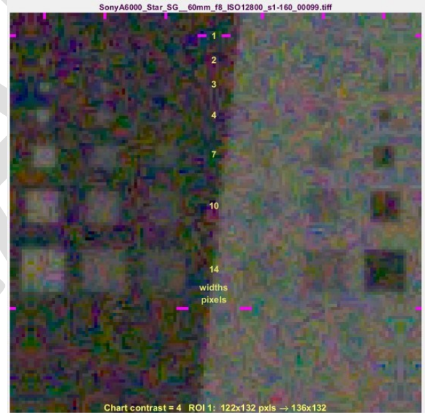
Figure 23. Noisy image, ISO 12800.
