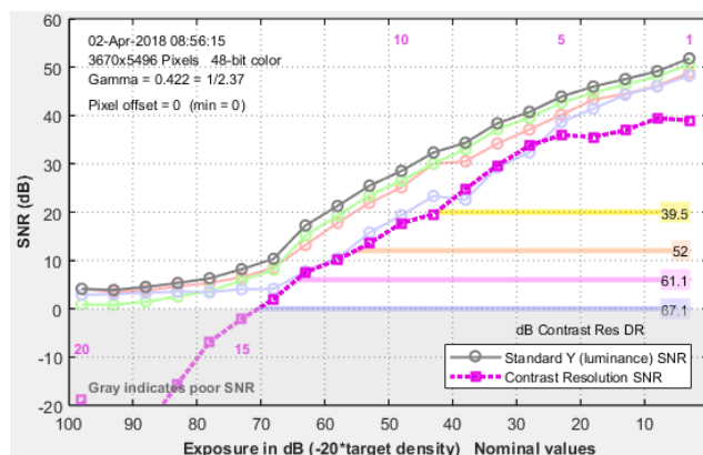
Contrast Resolution Dynamic Range, DR_{CR}
