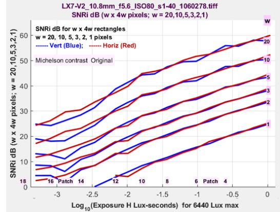
SNR_i for w \times 4w rectangles with w = 1, 2, 3, 5, 10 & 20 pixels for compact camera.
